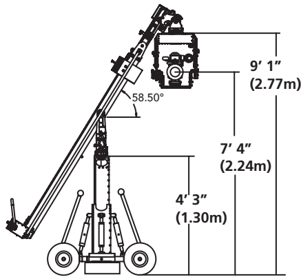
Underslung Retracted
