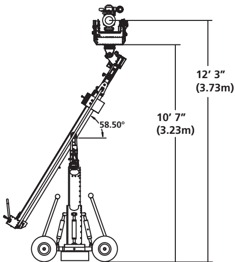
Overslung Retracted
