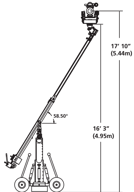
Overslung Extended
